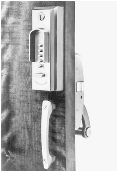
Figure 19.66 Unican 2000-15 unit used with an emergency exit panic bar. ( Simplex Access Controls Corp. )
