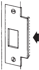
Figure 13.29 Bending strike.
