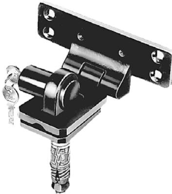
Figure 12.21 The Epilock high-security hasp and staple unit used the Mini Kaba cylinder. ( Kaba Locks, Ltd. )
