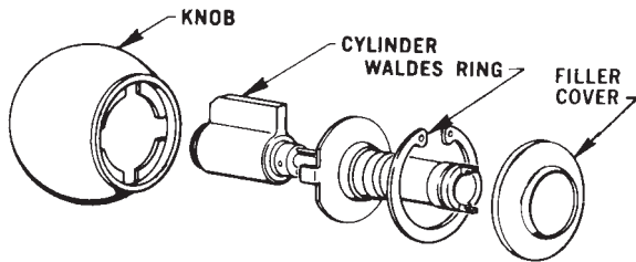
Figure 13.27 Removing cylinder.
