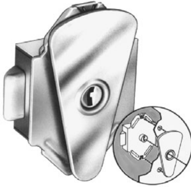
Figure 5.13 Series 6000 torsion tumbler lock with inset illustrating the snap-on face plate. ( Lock Corporation )
