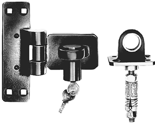
Figure 12.22 Epilok unit broken down into separate sections for installation. (Kaba Locks, Ltd.)
