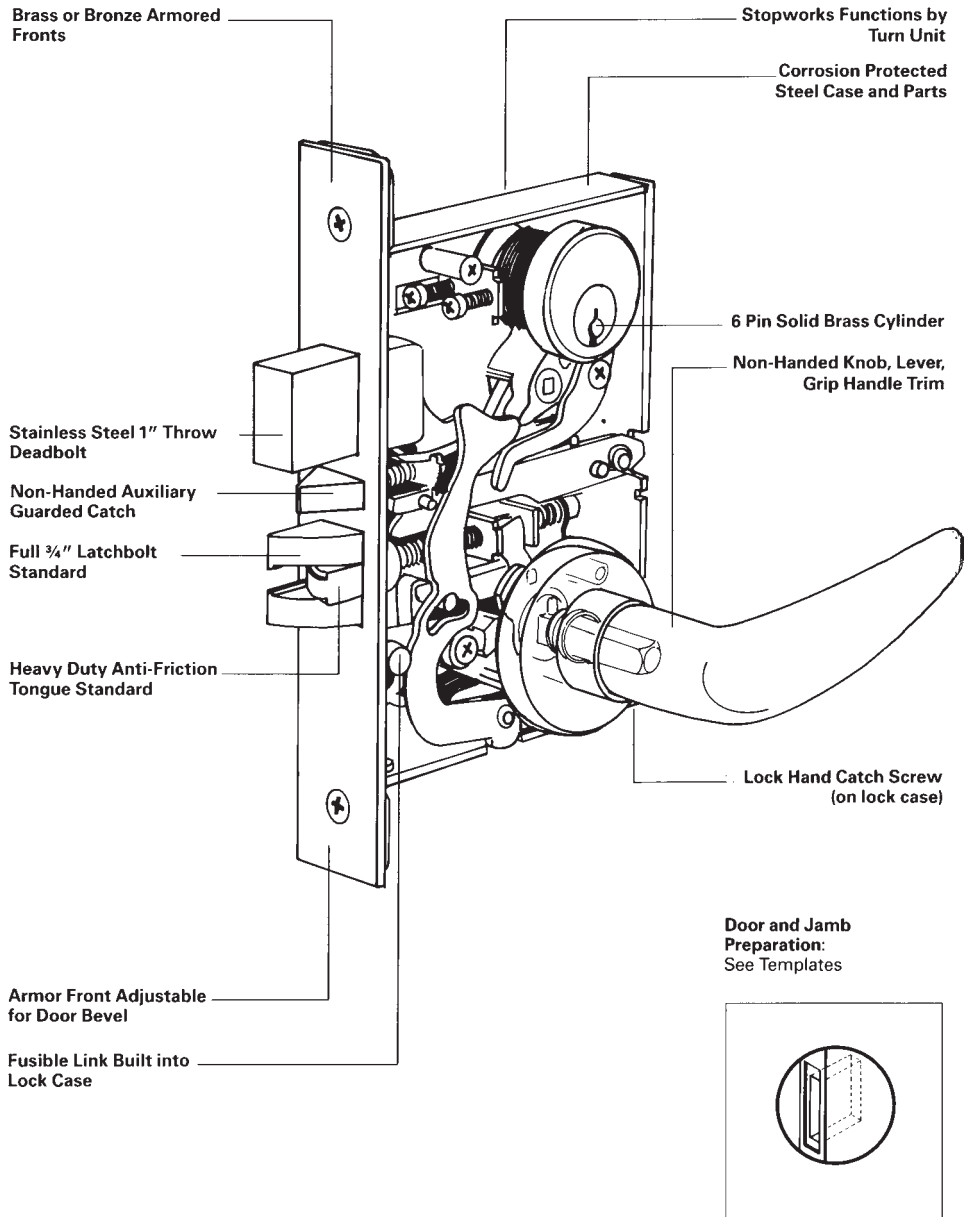
Figure 7.23 Schlage's L series mortise lockset. (Schlage Lock Company)
