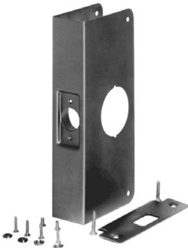
Figure 13.134 Install-A-Lock lock changing kit component parts. (M.A.G. Engineering and Mfg., Inc.)
