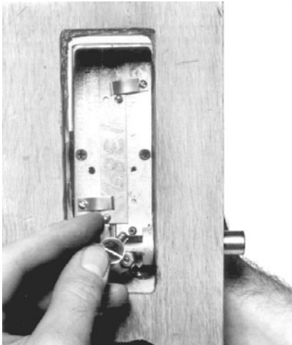
Figure 18.48 Preso-Matic installation, Step 2.
