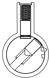
As change key rotates, construction wafer falls into "donut" hole in the side of plug. Only construction wafer will fall due to hole through its center.
