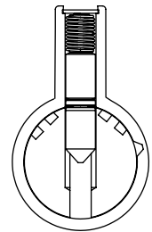
Change key inserted in cylinder putting the wafer at the shear line.
