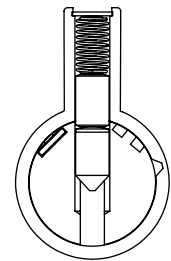
Construction master key inserted after wafer is trapped. Driver now extends into plug chamber. Construction master key, if used, will not rotate.
