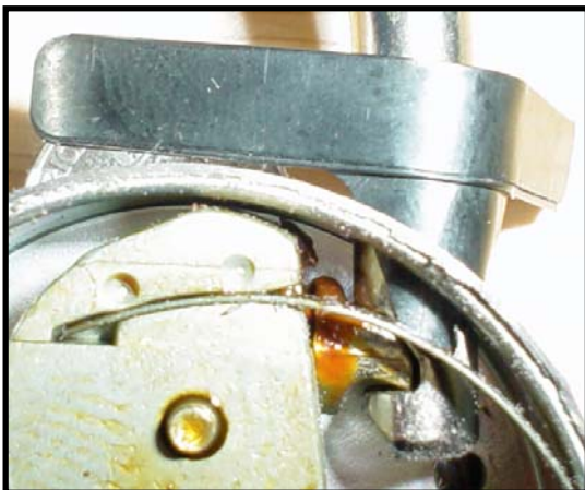
Locked – Bolt Extended/Shim Inserted.
