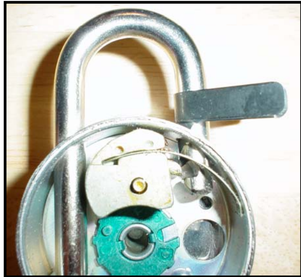
Unlocked – Bolt Retracted/Shim Turned.
