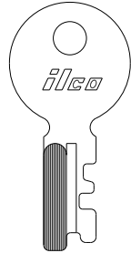
NICKEL SILVER .060" - 1.5mm .305" - 7.8mm 1326
