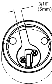
SARGENT standard cam shown
