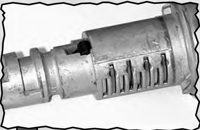
14 The cylinder plug uses a small actuator that must not be lost.
