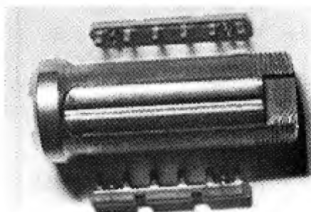
7...and two side bars found on the BiLock.
