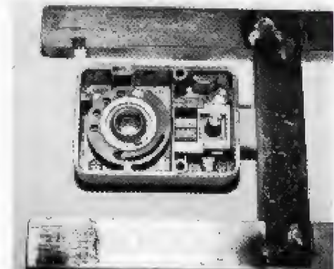
5. This is how the bolt and cross bolt assembly is installed on these locks.
