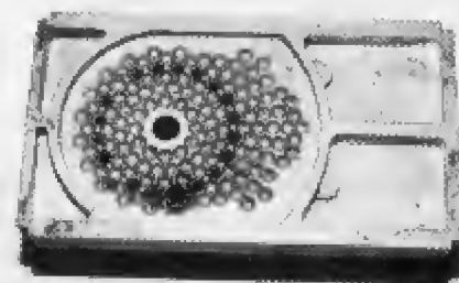
9. Ball bearings removed showing several through holes in the nest.
