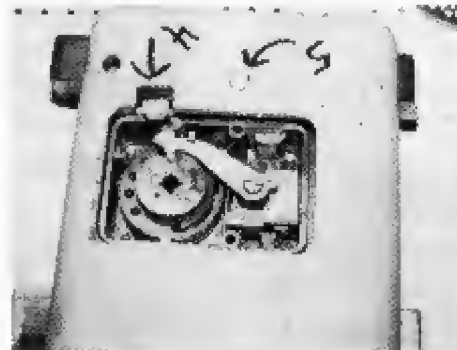
3. Inside view of non-servicable combination lock; #4 is the relock lever and #5 is the lever attaching rivet.
