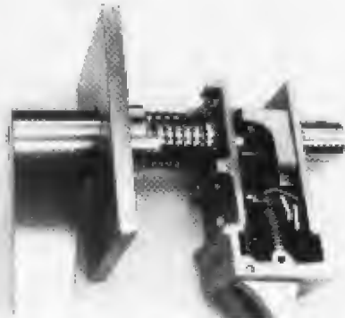
10. Assembly shown with the handle 180 degrees out of operating position.
