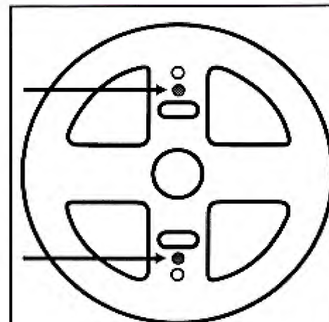
Illustration 1 Occasionally new holes have to be made in the standard S&G dial ring to accommodate the Mosler mounting screw location. (See arrows)
