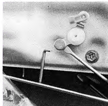
4. Moving the tool up to the bell crank.
