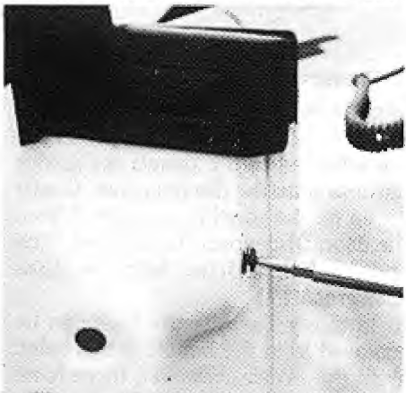
11. First handle screw is on door edge.
