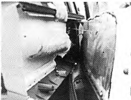
10. Before separating the panel from the door the lock, and latch rods, and a wire harness must be disconnected.
