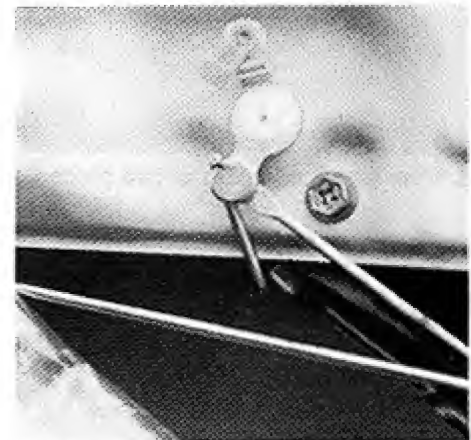
5. Pushing down on the bell crank opens the vehicle.
