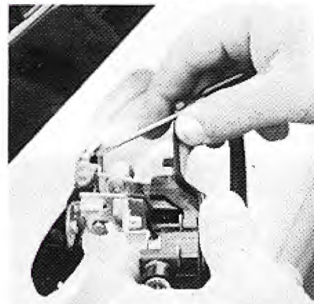
13. Disconnect the lock and latch linkage from the handle after it has been removed.
