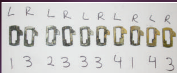
20. The door lock contains all cuts and the wafers are stamped. Laying the wafers out in order we must remember the rule; Left-Right-Left-Right....
