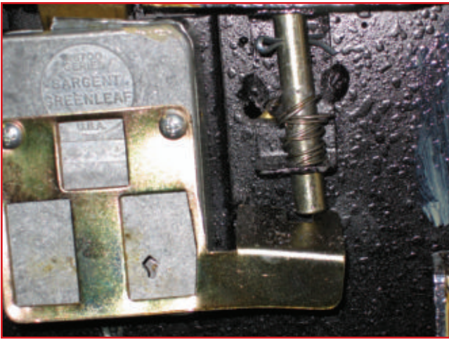
7. Spring destroyed on relock pin held up by relock activating plate.
