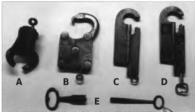
6. The Crabclaw (A), an early Yale prototype (B), a prototype slider by J.C. Preston (C), a production slider (D), and keys (E) for Yale Quadplex and rim lock.
