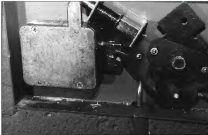
5. Locking plate bypassing the lock bolt opening safe door.
