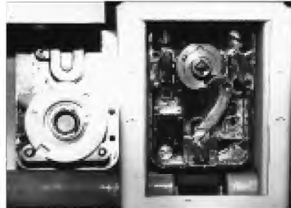
10. The opened lock. A drilled hole can be seen through the lock case and in the end of the lever.
