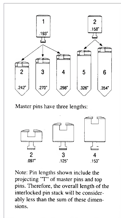
7. Notice the interlocking "T" shape of the bottom and master pins.
