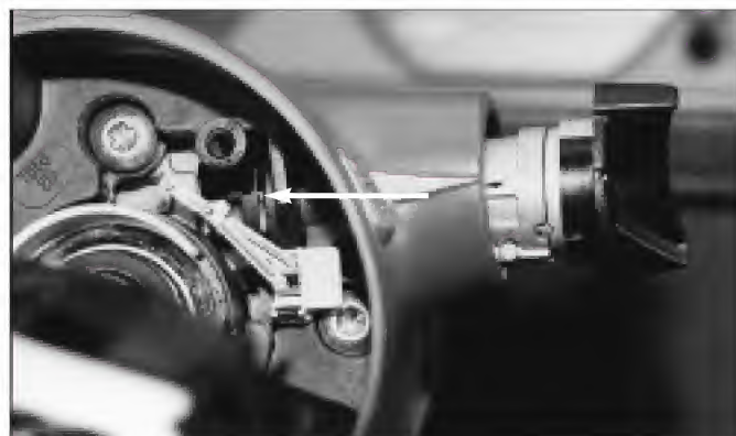
6. This small slot serves to hold the ignition lock retainer. Depress the retainer and slide the lock out of the column.
