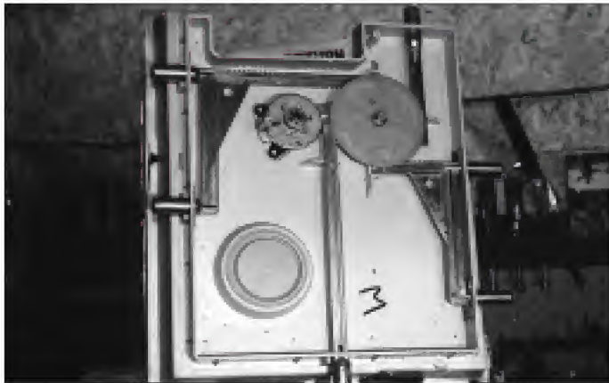
9. Inner bolt and wheel pack configuration of Sentry Door. Bolts are geared. Large plastic wheel has gears on back.
