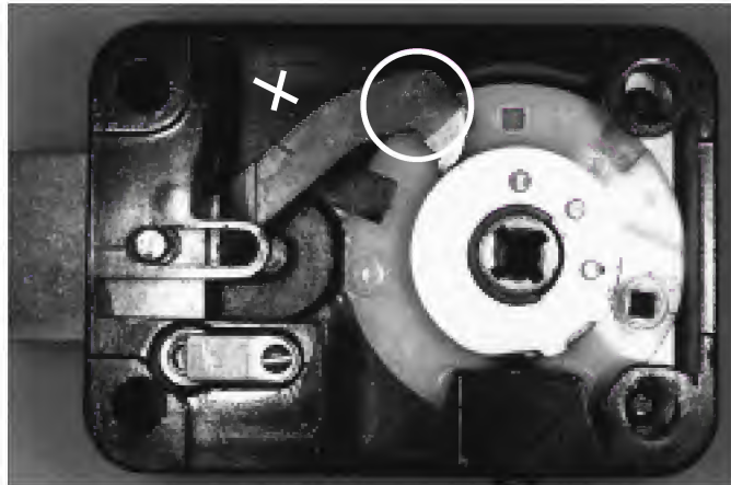
4. An X-ray view of the Mosler 302 lock. The circle is drill area for the fence. The X is a secondary scope location.
