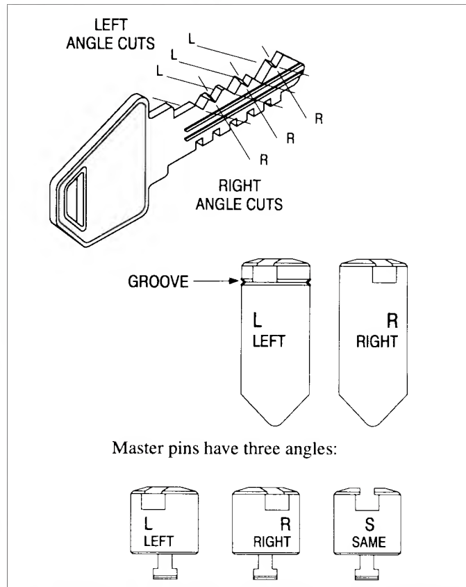
3. In order to operate, the pins in the lock must not only be cut with the correct depth, they must also have the correct angles.
