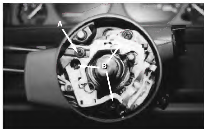
5. Remove the turn signal lever screw (A), and the three turn signal mounting screws (B).
