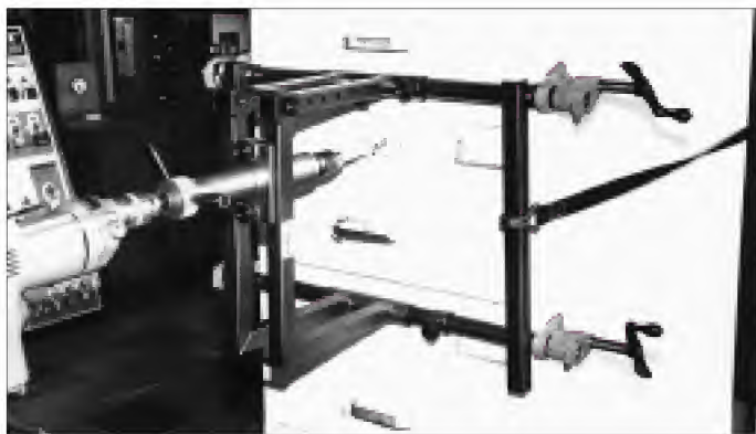
2. The fixed drilling rig - A Magnum 357.
