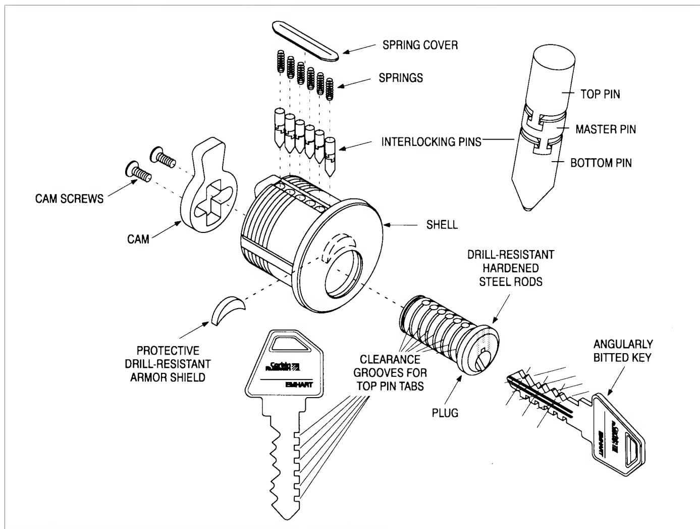
1. Exploded view of the Corbin Russwin High Security cylinder.
