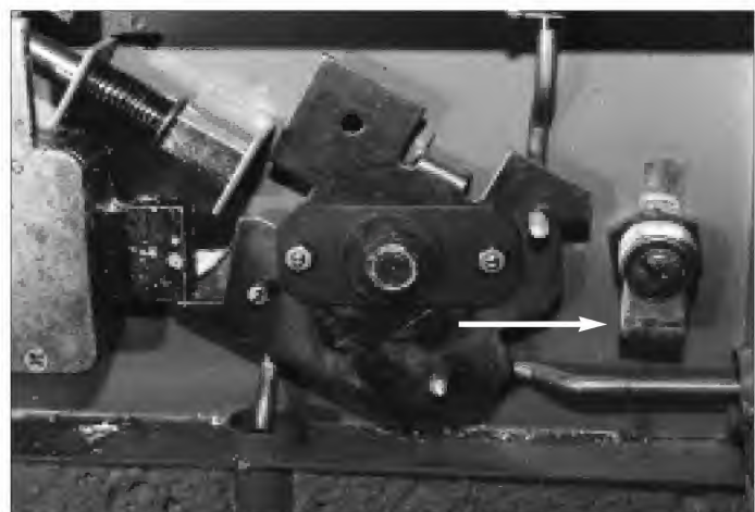
4. Cam lock in the open position. This will allow the locking plate to turn.
