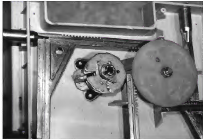
10. Close up of wheel pack and geared locking bolts.
