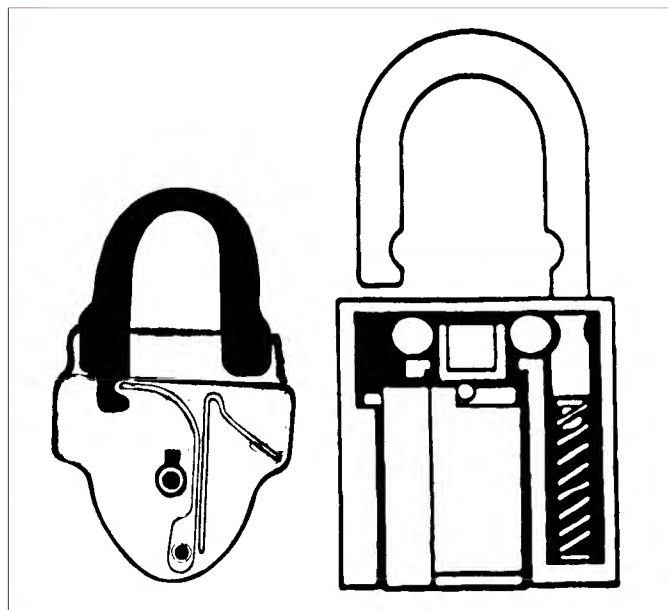
4. Through the years, padlock design and application have remained similar. On the left is a representational view of an ancient padlock. To the right, a more current padlock representation.
