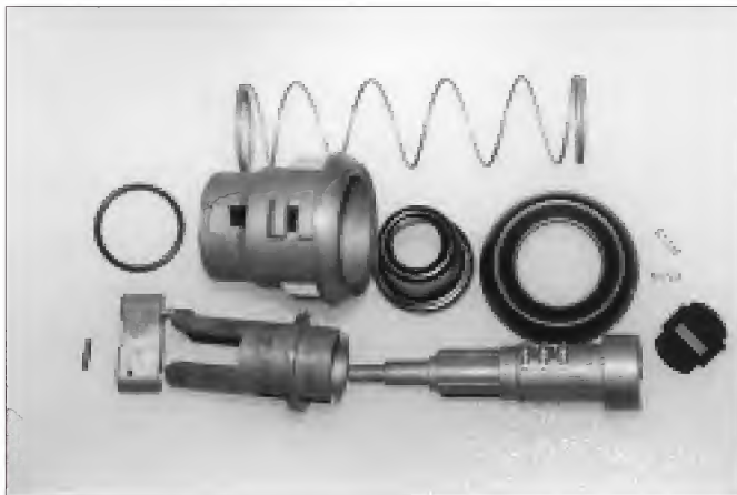
16. The tailgate lock is easier to replace than to rebuild. This service kit is available from Briggs & Stratton.
